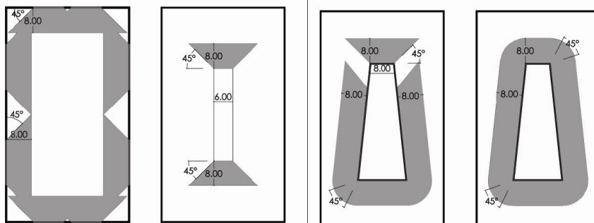
Diagram 2: Models showing possible building floor plates. Left model showing how windows are to be considered on the floor plate. The three to the right illustrate various atria; shaded areas are those areas that meet the Credit Criteria.
