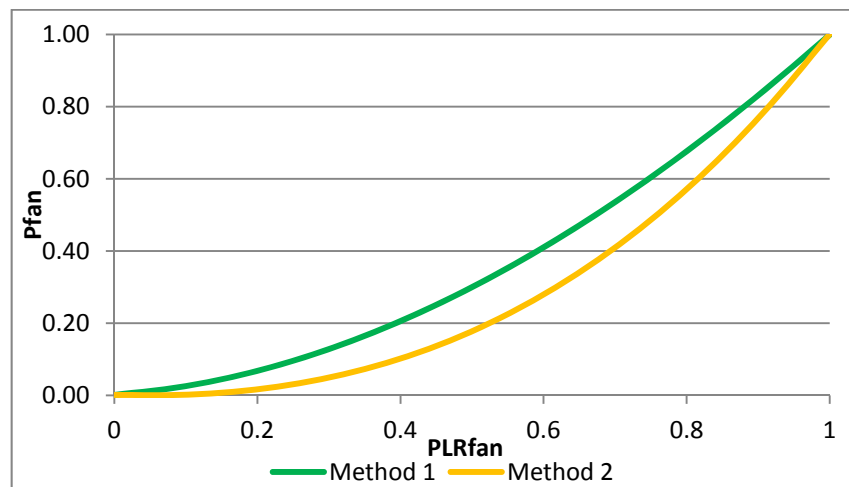
Figure 1: Proportion of full-load fan power for Method 1 and Method 2
