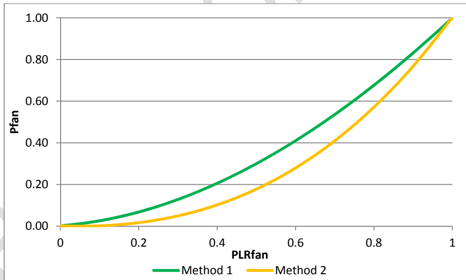
Figure 1: Proportion of full-load fan power for Method 1 and Method 2
